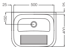
Pileta para lavadero acero inoxidable para sobre o bajo poner Under or over counter stainless steel laundry basin G4400 AS / AB
