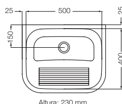
Pileta para lavadero acero inoxidable para amurar Wall mounted stainless steel laundry basin G4401 AS / AB
